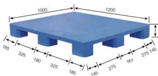
名称: 21#平面九脚卡板 Product Name: 21# Flat Pallet 材质: PP Material: PP 规格: 1200x1000x140 Size: 1200x1000x140 颜色: 黑色/蓝色 Color: Black/blue
