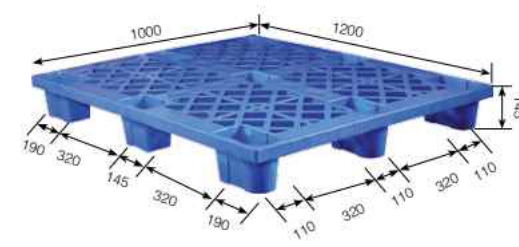
名称: 54#网格九脚卡板 Product Name: 54# Grid Pallet 材质: PP Material: PP 规格: 1200x1000x140 Size: 1200x1000x140 颜色: 黑色/蓝色 Color: Black/blue
